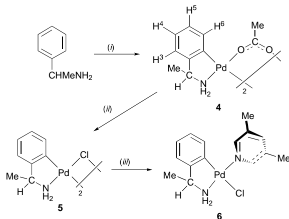
Scheme 2 (i) \text{Pd}(\text{O}_2\text{CMe})_2 ; (ii) \text{NaCl} ; (iii) dmpy
