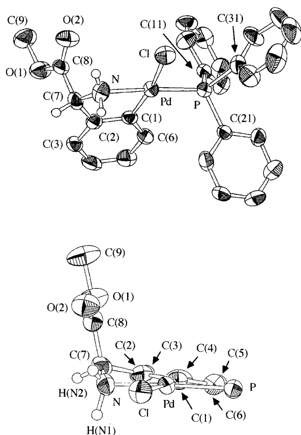
Fig. 1 Molecular structure of [\text{PdCl}(\text{C}_6\text{H}_4\text{CHCO}_2\text{MeNH}_2)(\text{PPh}_3)] 3
